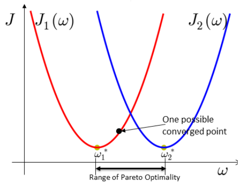
Figure 1 Two tasks with different optimal value w_1^* and w_2^* . The network will finally converge to some point w between w_1^* and w_2^* . Obviously, any attempt to decrease one task's loss lies at the cost of increasing the other's (e.g., moving w down along the red line increases J_2(w) ).
