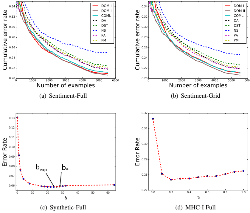
Figure 2 Above is the learning process on Sentiment dataset; below is the parameter effect on Synthetic and MHC-I dataset.
